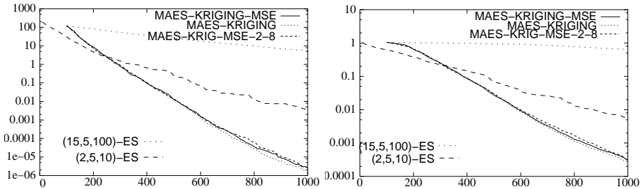
Figure 2: Average plots of 20 runs on sphere function. Fitness value (right) and the global step-size (left) vs the number of exact evaluations.
