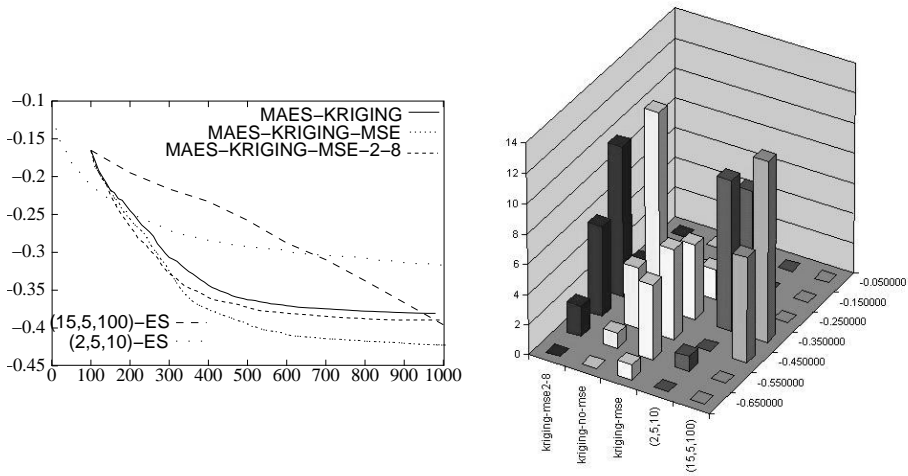
Figure 4: Results on 20 dimensional Keane Function using the Kriging approximator: Averaged fitness histories for 20 runs (left) and a histogram for the best found values in the 20 runs after 1000 exact evaluations (right) are plotted.
