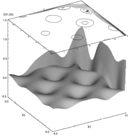
Figure 3: Keane's function plotted in 2-dimensions for a cut of the search space. The optimum is indicated by the black spot in the upper right corner of the contour plot.
