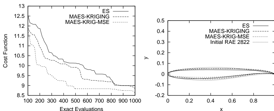
Figure 5: Left: Average convergence histories of 3 runs of the airfoil shape optimization problem with the ES and MAES using one and both selection criteria. Right: Initial airfoil profile and the optimal ones computed using ES and MAES.
