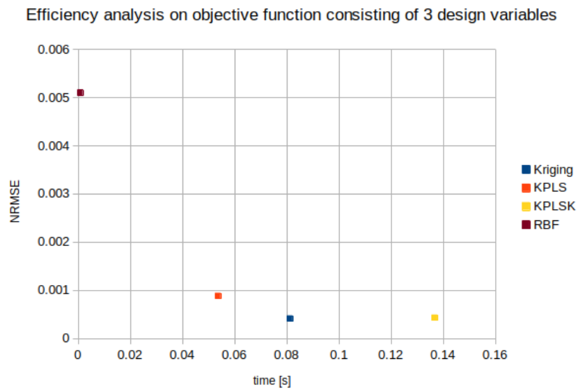
Figure A.1: Efficiency analysis on eq. A.2
