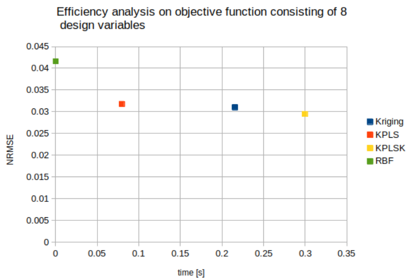
Figure A.2: Efficiency analysis on eq. A.3
