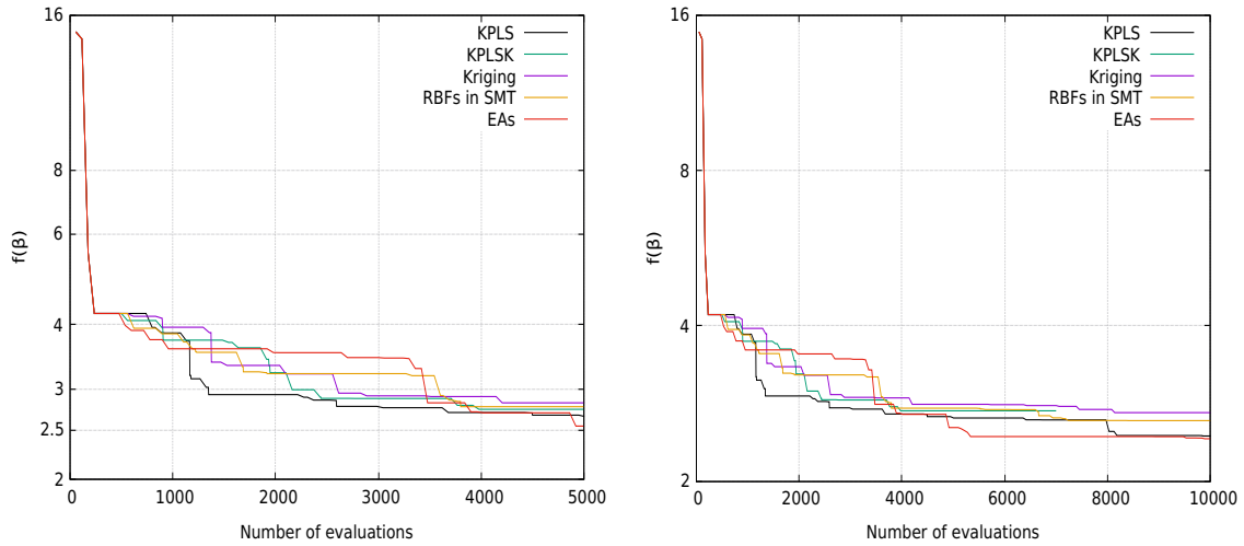
Figure 5.9: Welded beam design with RNG1. Comparison between the convergence history of EAs and MAEAs with metamodels trained on-line via SMT
